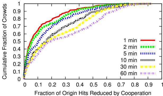
Figure 5: Origin load reduction from cooperation, as a fraction of total requests, for crowds defined by different epoch lengths.
